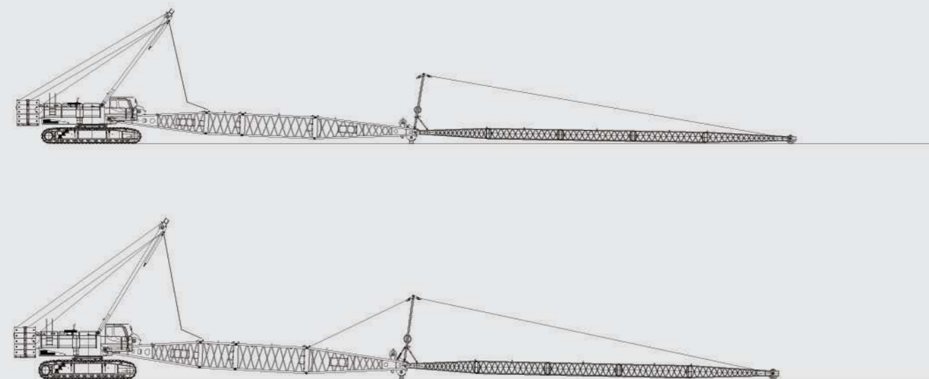
固定副臂安装示意图 Fixed Jib Installation Illustration
